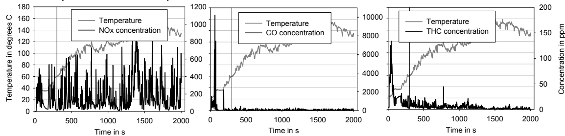
Figure 31: Cold start exhaust pollutant concentrations of Euro 5 diesel Vehicle H
