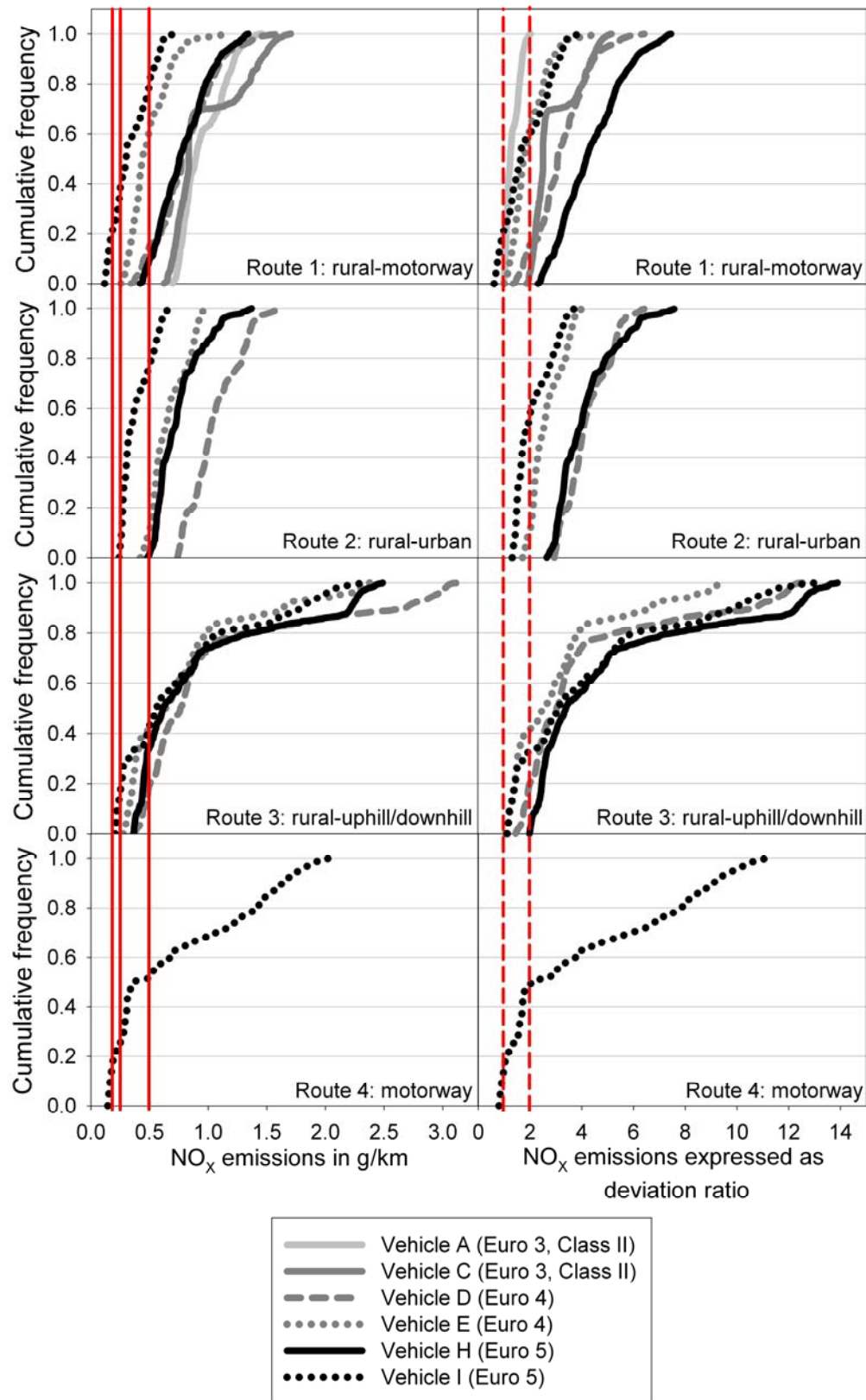
Figure 27: Comparison of the averaging window NO x emissions of Euro 3-5 diesel vehicles on the four PEMS test routes; red solid lines indicate from left to right the Euro 3-5 emission limit; Euro 3 and Euro4 Class II emission limits for Vehicle A and C correspond to 0.65 g NO x /km and 0.33 g NO x /km, respectively and are not indicated for reasons of simplicity; red short-dashed lines indicate from left to right the factor one and two of the respective Euro 3-5 emission limit
