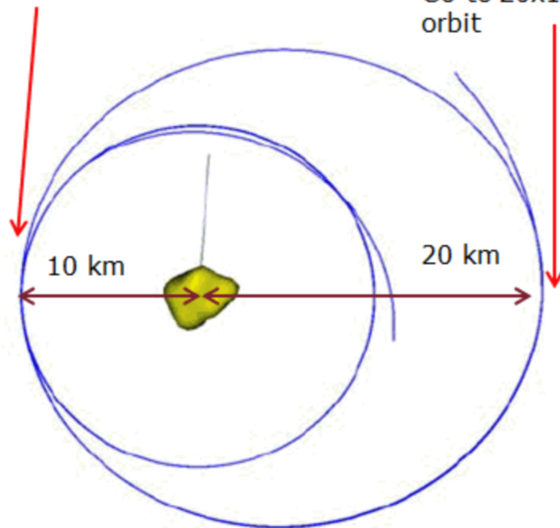
Comet and orbits seen from Sun direction
