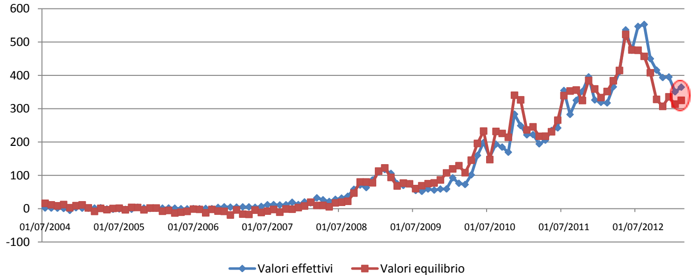
Equilibrium vs Effective BTP-BUND Spread 10Y - Spain
